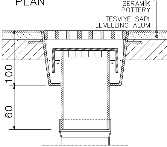
KESİT SECTION
