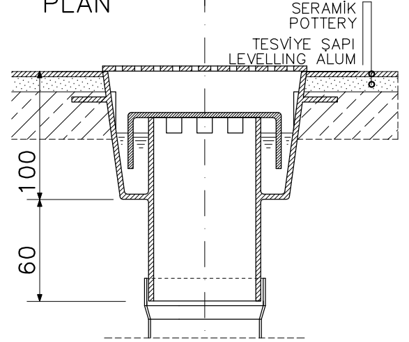
KESİT SECTION
