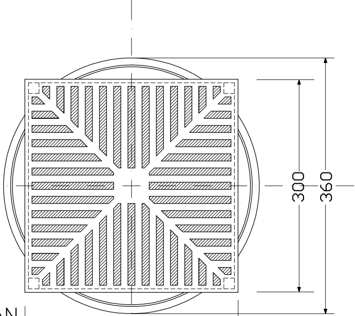
DÜZ KARE İZGARA FLAT SQUARE GRID
