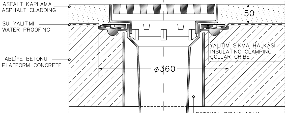
KESİT/SECTION
