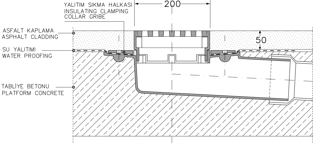
KESİT/SECTION
