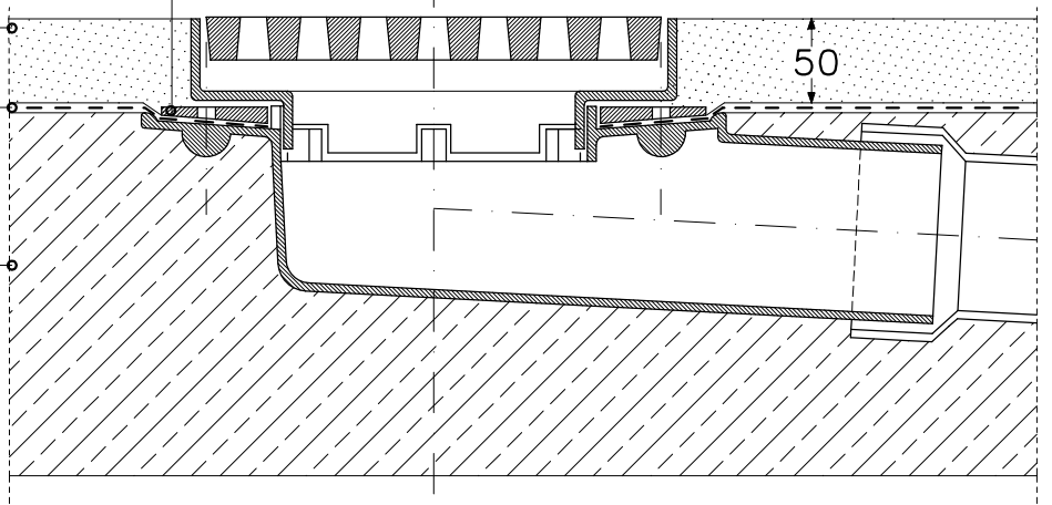
YALITIM SIKMA HALKASI INSULATING CLAMPING COLLAR GRIBE
