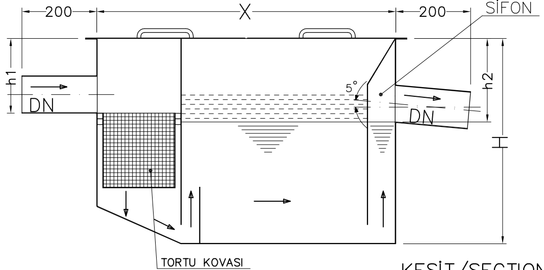
KESİT/SECTION
